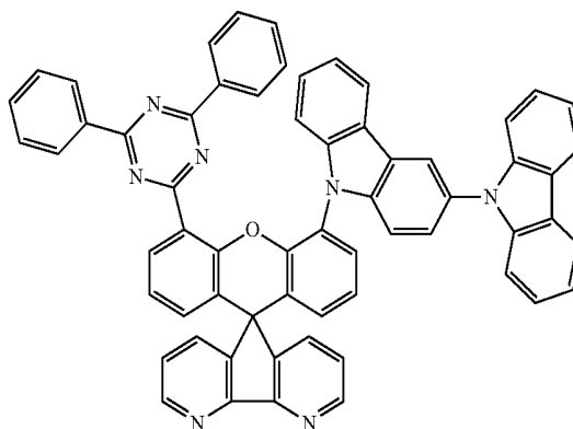
compound 28
