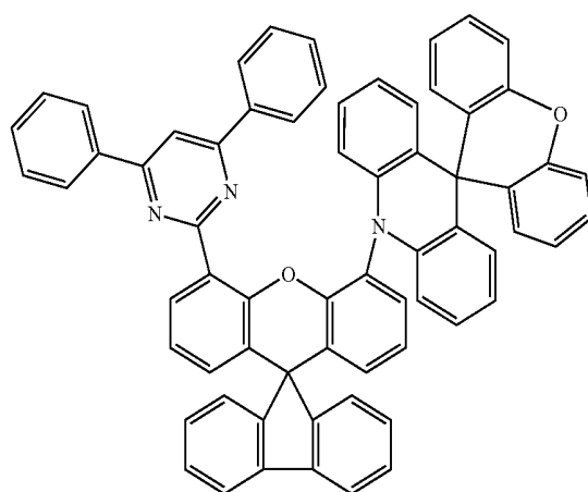
compound 6
