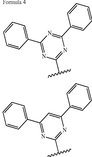
Formula 4
