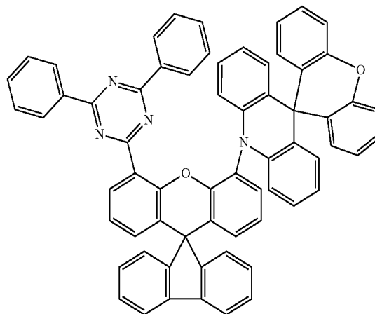
compound 2
