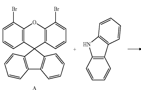
Reaction Formula 1-3
