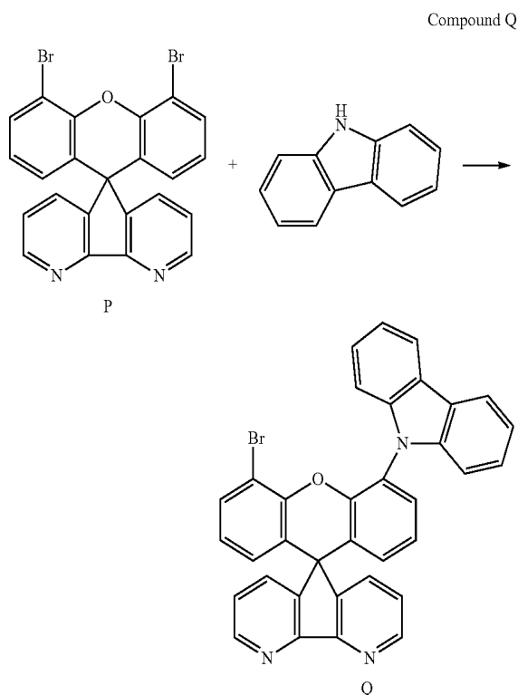
Reaction Formula 6-2
