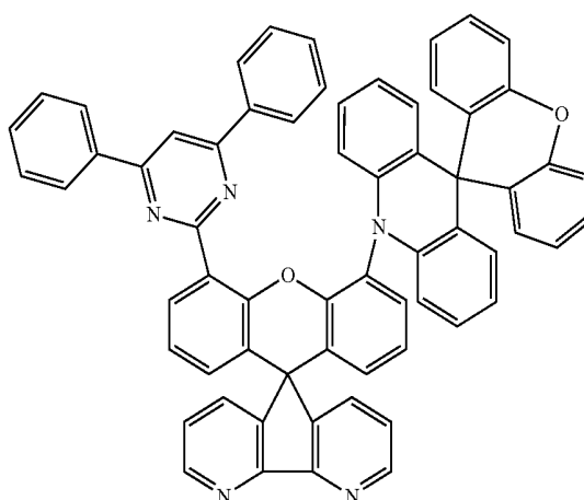
compound 30
