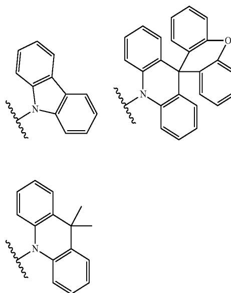
Formula 5
