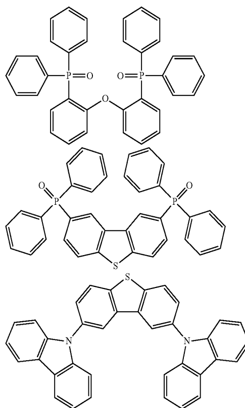
Formula 10
