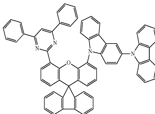
compound 8
