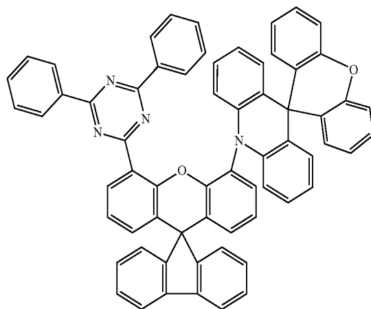
compound 2
