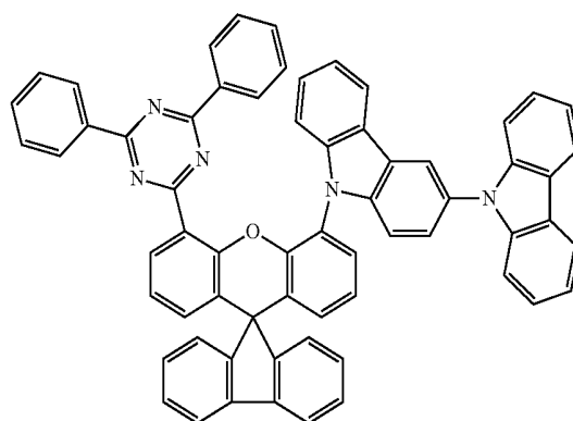
compound 4
