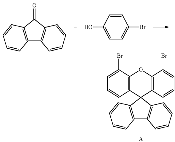
Reaction Formula 1-1
