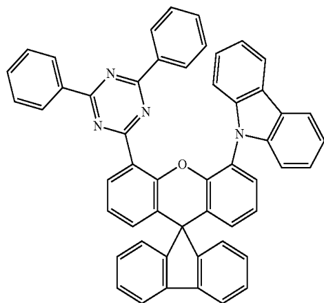
Formula 6
