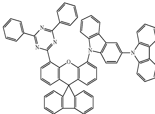
compound 4
