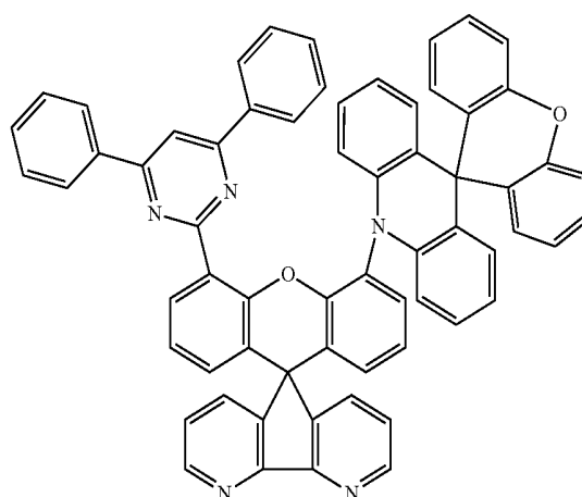
compound 30
