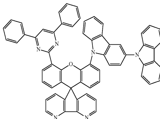
compound 32
