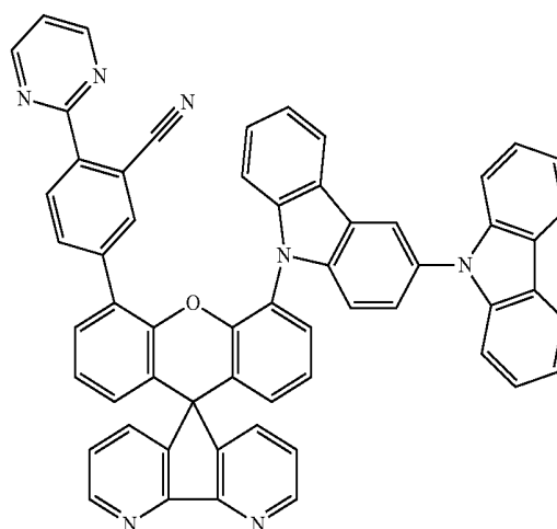
compound 36
