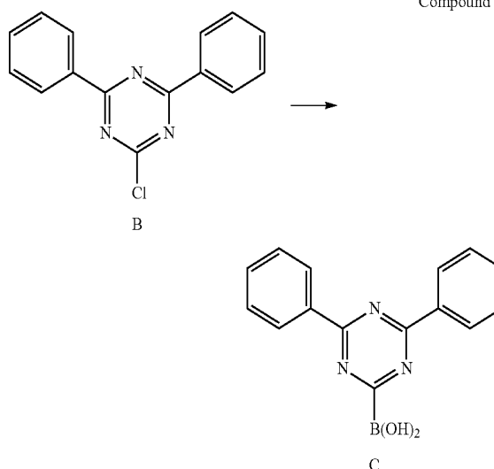
Reaction Formula 1-2
