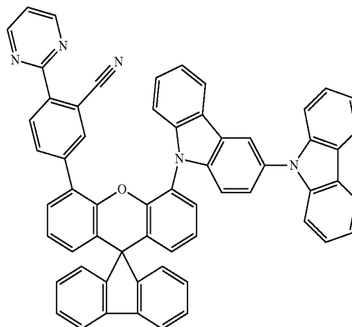
compound 12
