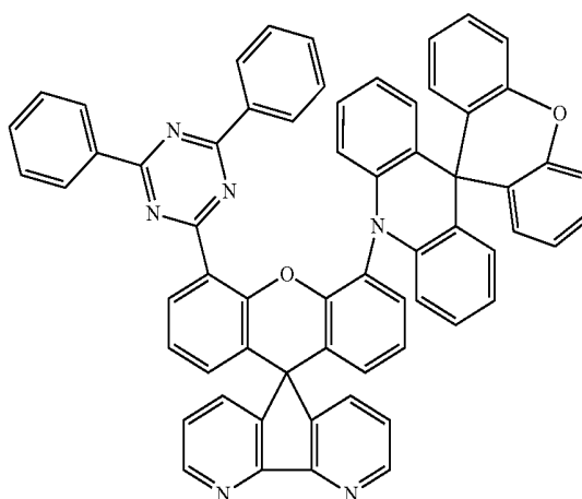
compound 26
