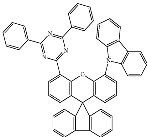
Formula 6
