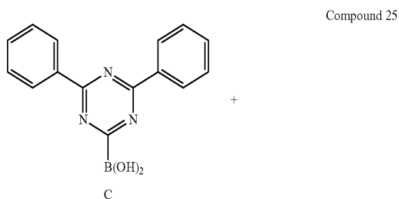
Reaction Formula 6-3
