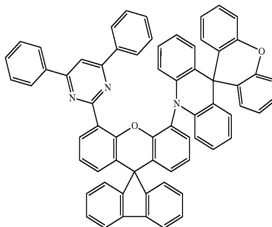
compound 6
