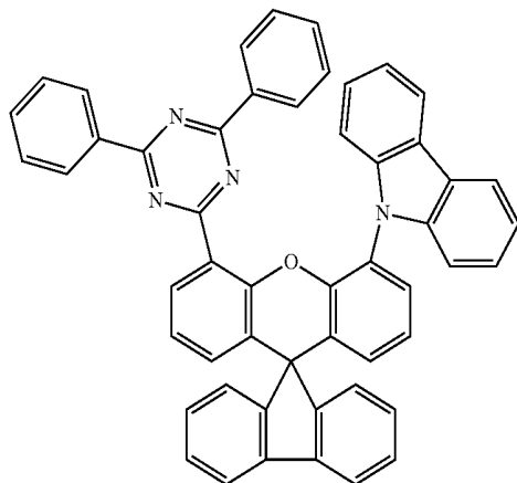
Formula 6
