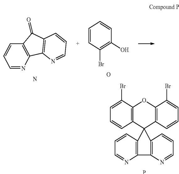
Reaction Formula 6-1
