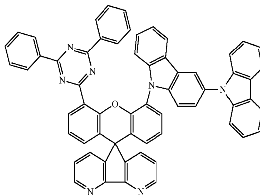
compound 28
