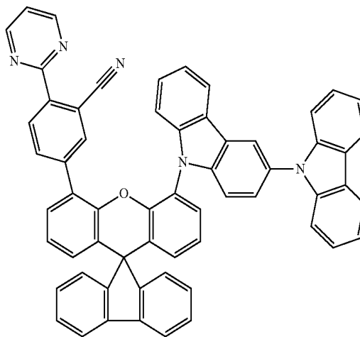
compound 12
