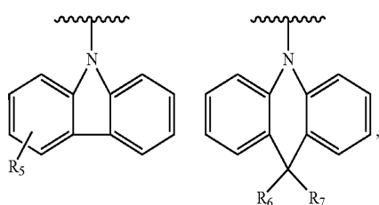
Formula 3
